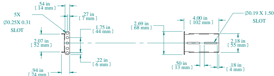
SLIDE RAIL MOUNT BRACKETS
